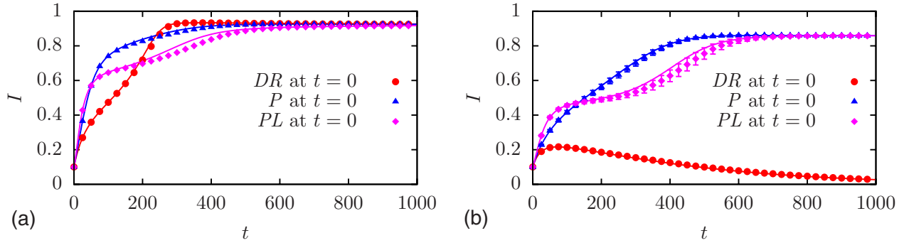
FIG. 2. (Color online) Disease prevalence I against time t on networks featuring the same mean degree \langle k \rangle = 2 but different initial degree distributions ( p_k^{DR} , p_k^P , and p_k^{PL} ). Parameters are (a) \beta = 0.06 , \gamma = 0.02 and (b) \beta = 0.04 , \gamma = 0.04 . We use \alpha = 0.005 and \epsilon = 0.1 in all simulations. Points and error bars (if larger than marker size) correspond to the mean and standard deviation computed over 10 000 Monte Carlo simulations; solid lines are the predictions of our analytical approach.
