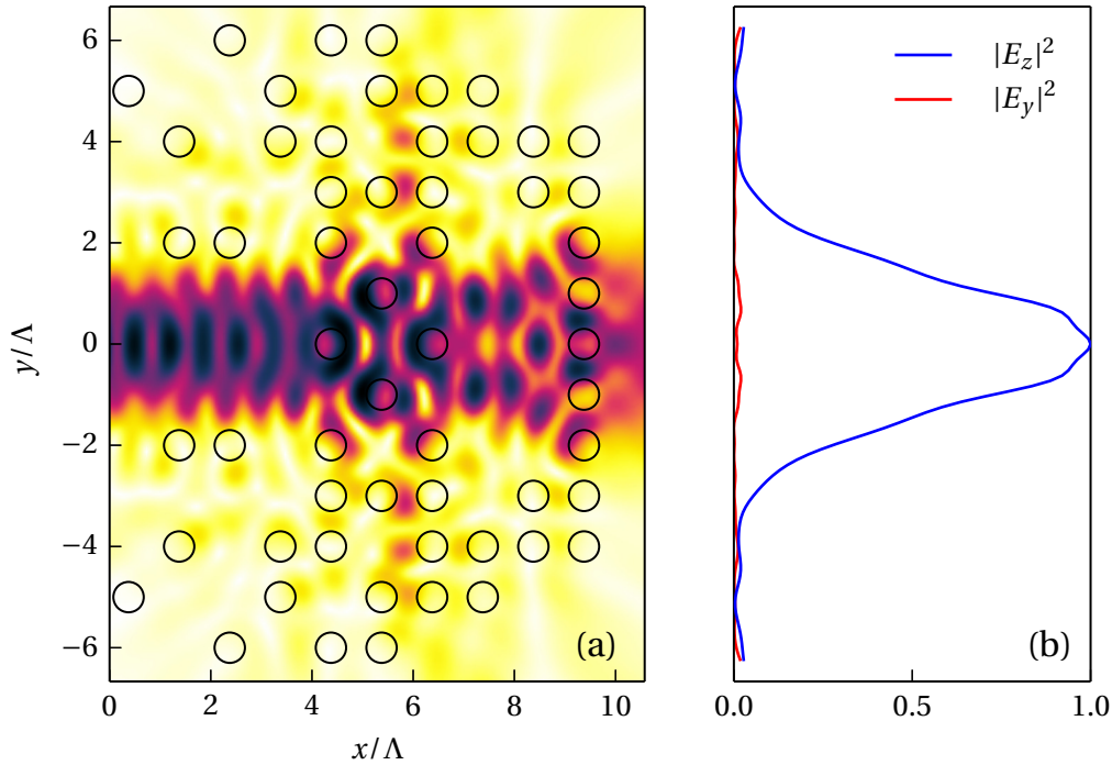
Figure 6.3 – Generation of a TM polarized Gaussian beam. (a) Optimized HIS configuration (57 scatterers) and |E_z| field profile (arbitrary units). The target plane coincides with the upper limit of the x axis. (b) Comparison of orthogonal polarization components along target plane. This solution is characterized by \mathcal{P} = 0.983 , R = 59.8 , g = 0.044 , \eta = 0.759 .
