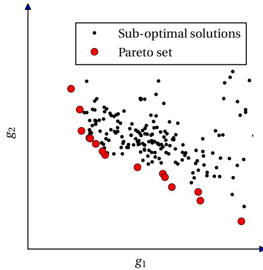
Figure 3.5 – Typical Pareto front of a biobjective optimization problem. Black dots indicated dominated solutions, as for each of these solutions, there exists a solution characterized by a better value of both g_1 and g_2 . Real data taken from Fig. 5.11.
