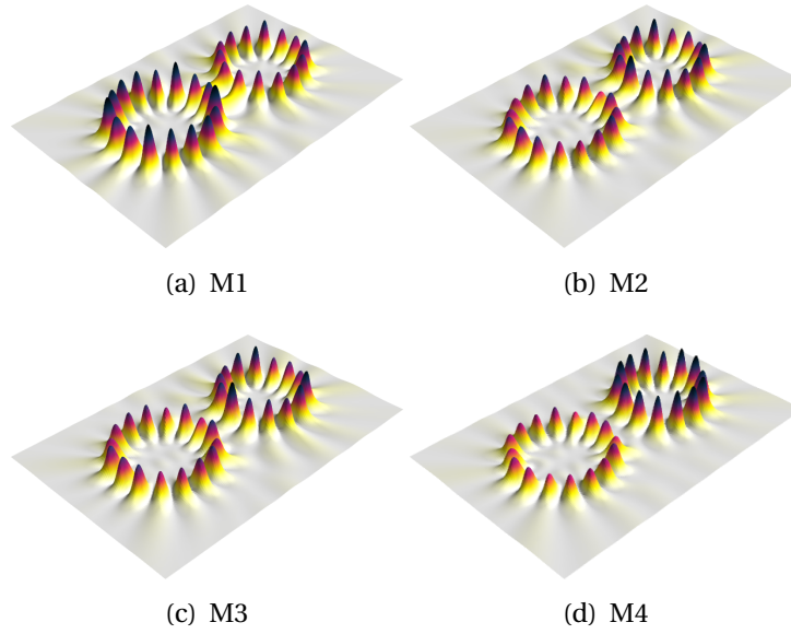
Figure 7.2 – Profile of four TM-polarized QB states of a diatomic photonic molecule composed of two cylinders of different diameters, as shown in Fig. 7.1. The z -coordinate is proportional to the intensity (arbitrary units).
