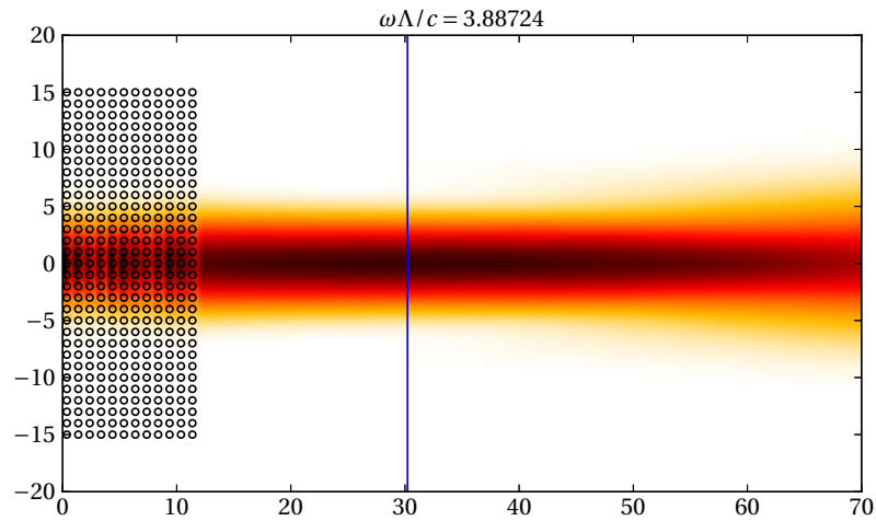
(b) \mathcal{D} < 0
