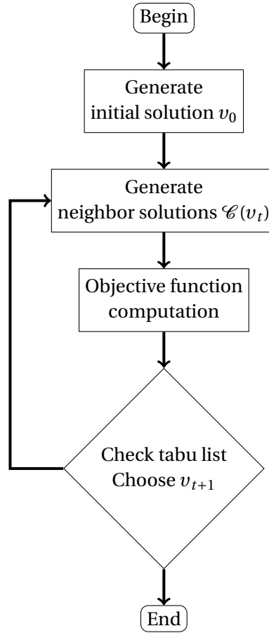
Figure 3.3 – High-level template of tabu search [149].
