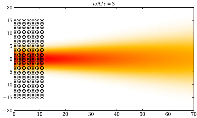
(a) \mathcal{D} > 0
